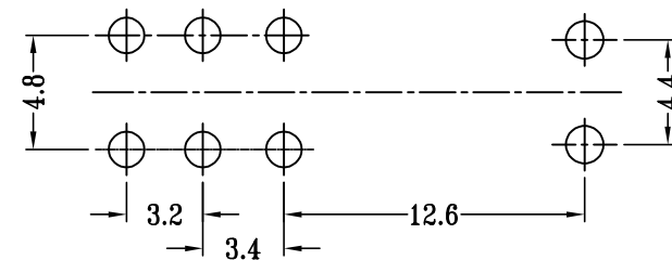
P.C.B LAYOUT BOTTOM VIEW
