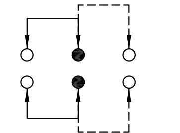
SCHEMATIC (NON-SHORTING)
