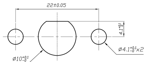
PANEL CUTOUT
