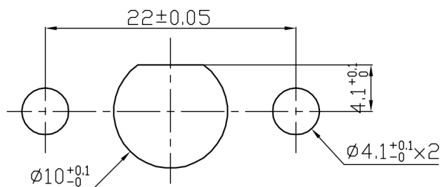
PANEL CUTOUT
