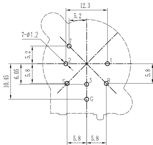
P. C. B LAYOUT (TOP VIEW) Tolerance: \pm 0.05
