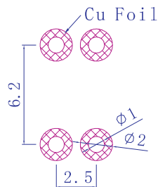
PCB Hole Layout
