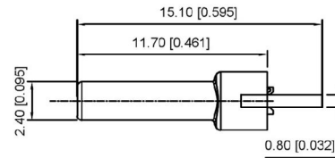
SECT B-B
