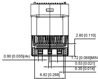
SECT B-B
