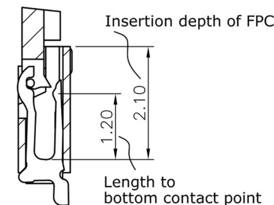
SECTION VIEW SCALE 10/1
