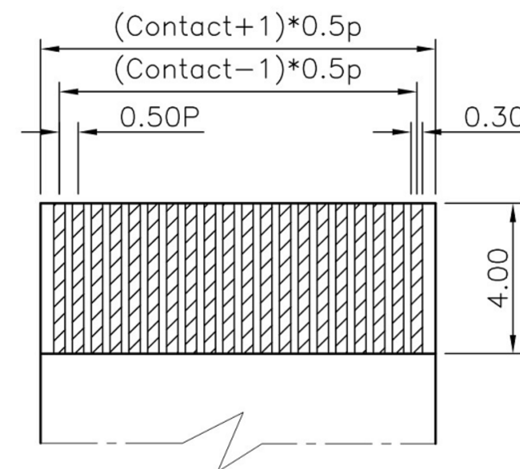
FFC/ FPC DIMENSION THICKNESS 0.3mm
