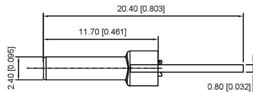
SECT B-B
