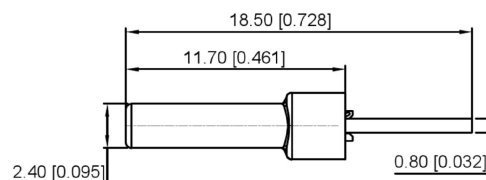
SECT B-B
