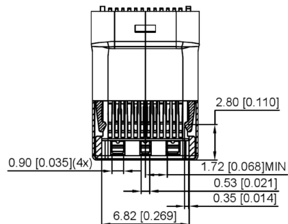
SECT B-B
