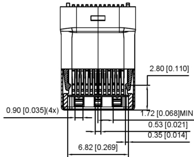
SECT B-B
