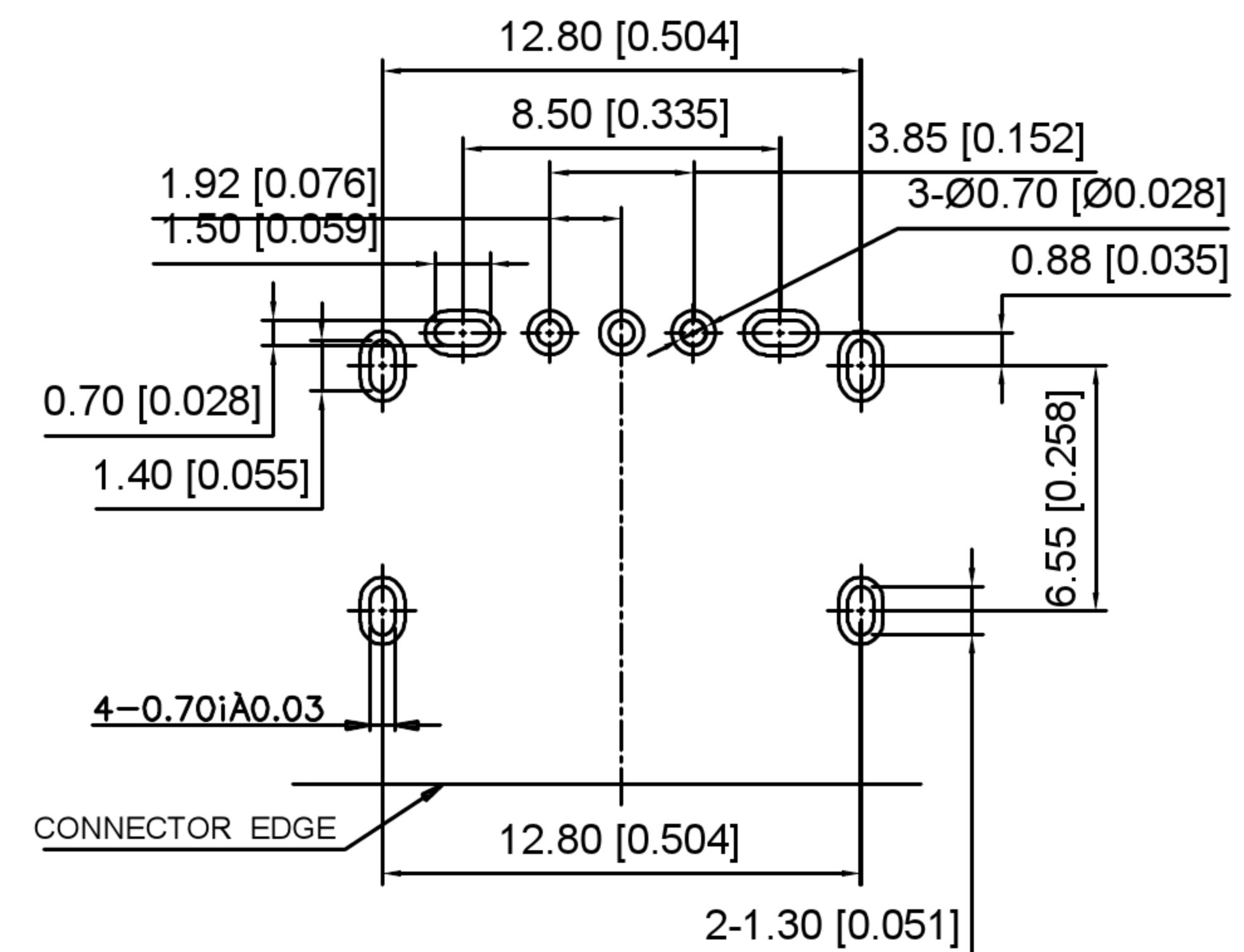
RECOMMENDED PCB LAYOUT(THK:1.0MM)
