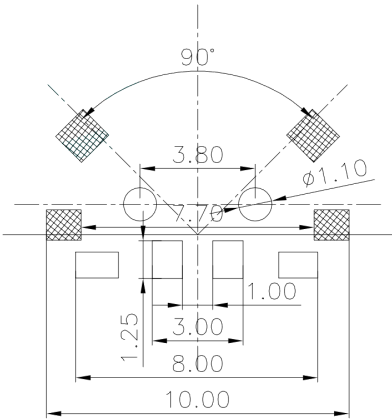
P.C.B Mounting Pattern Dimension
