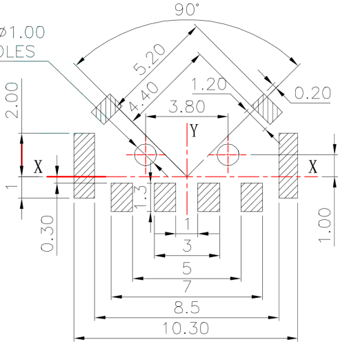
P.C.B Mounting Pattern Dimension
