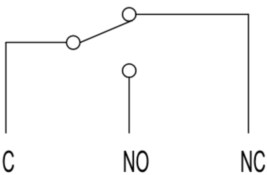
SCHEMATIC
