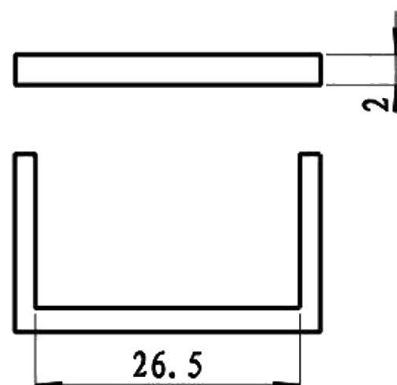
PANEL CUT-OUT
