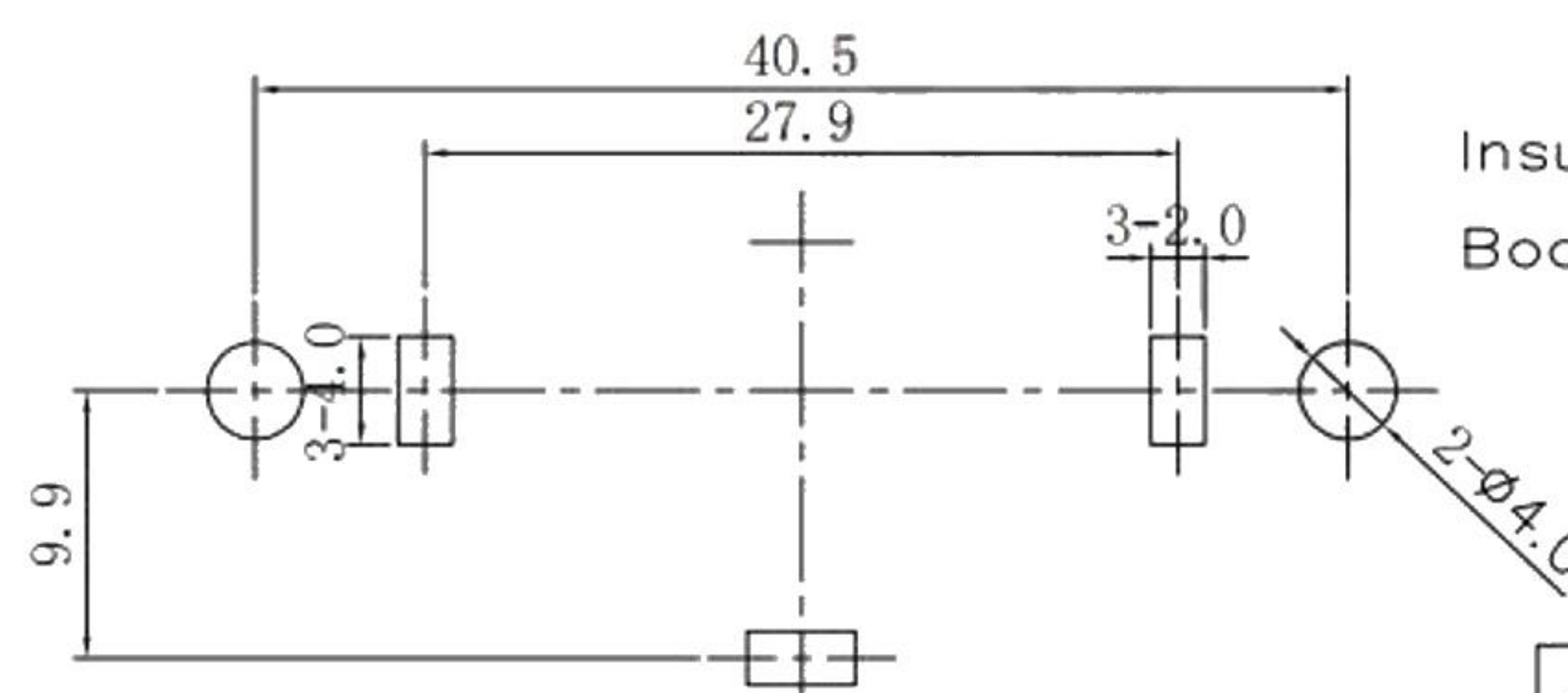
PANEL CUT-OUT
