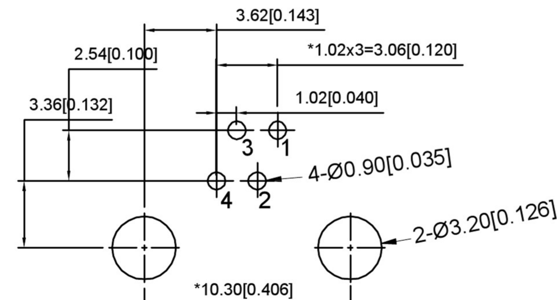
RECOMMENDED PCB LAYOUT VIEWED FROM COMPONENT SIDE
