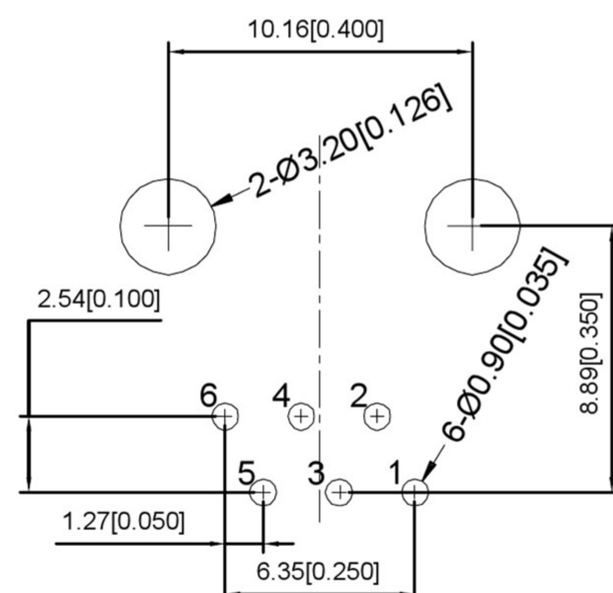
RECOMMENDED PCB LAYOUT VIEWED FROM COMPONENT SIDE
