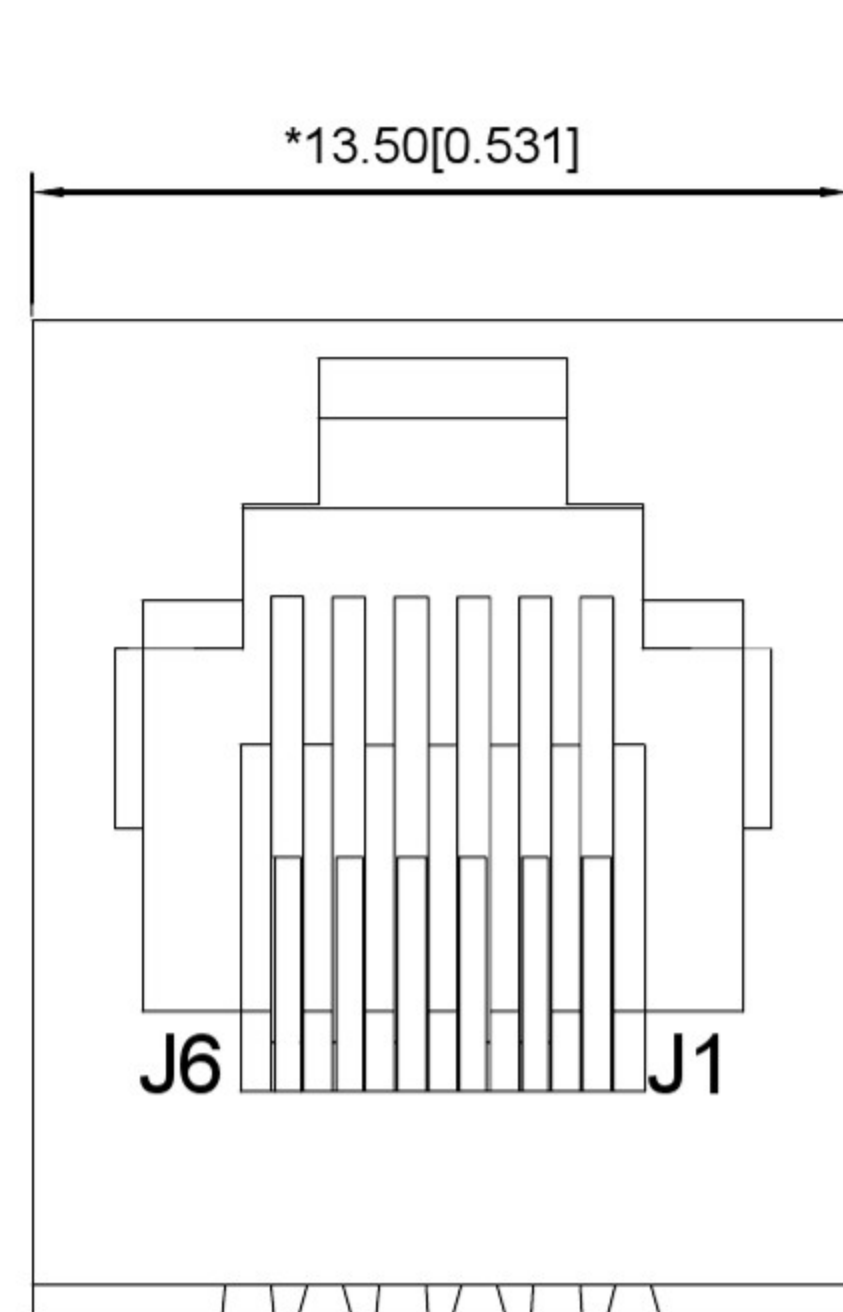
FRONT VIEW
