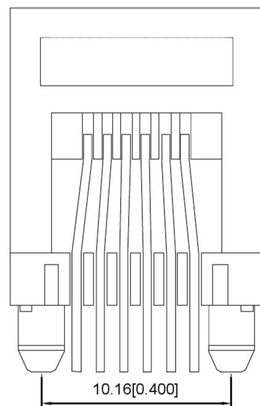
BACK VIEW
