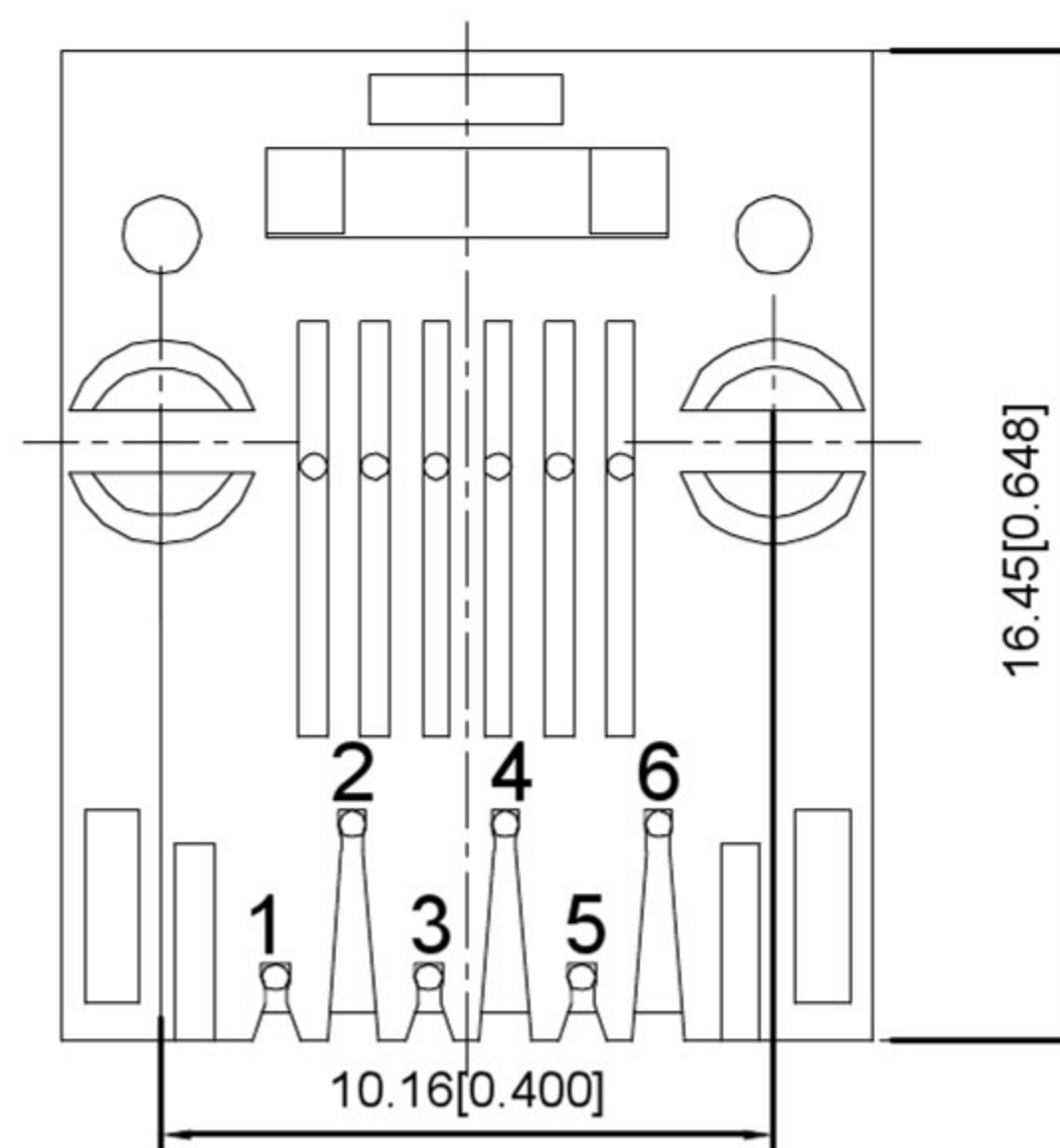
BACK VIEW
