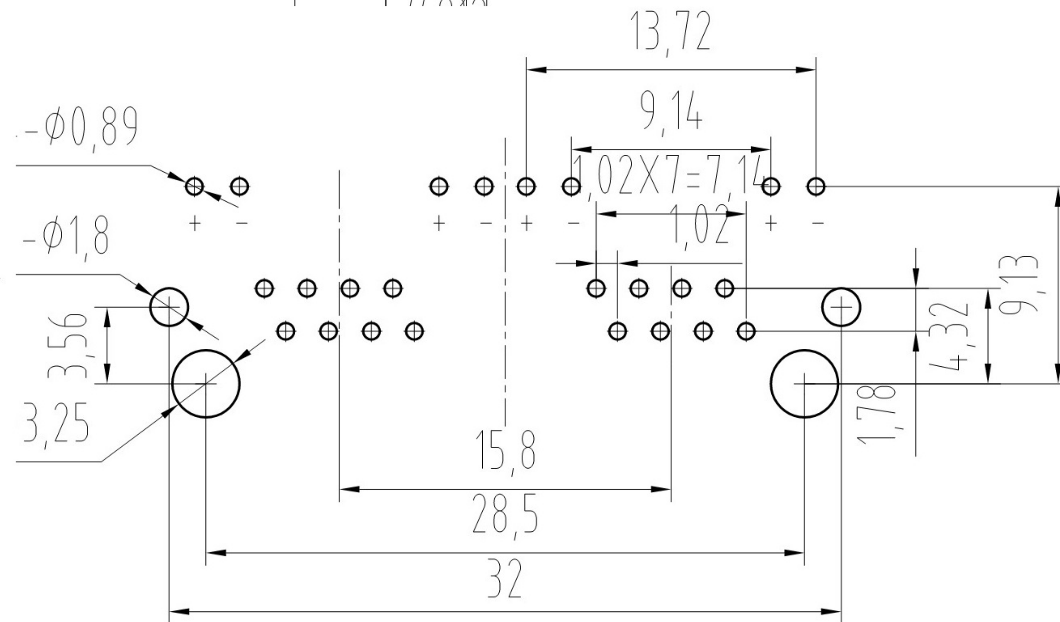
PC Board Layout Component Side Shown
