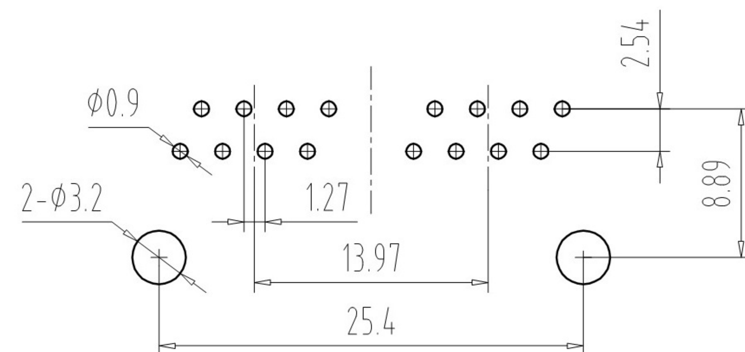
PC Board Layout Component Side Shown
