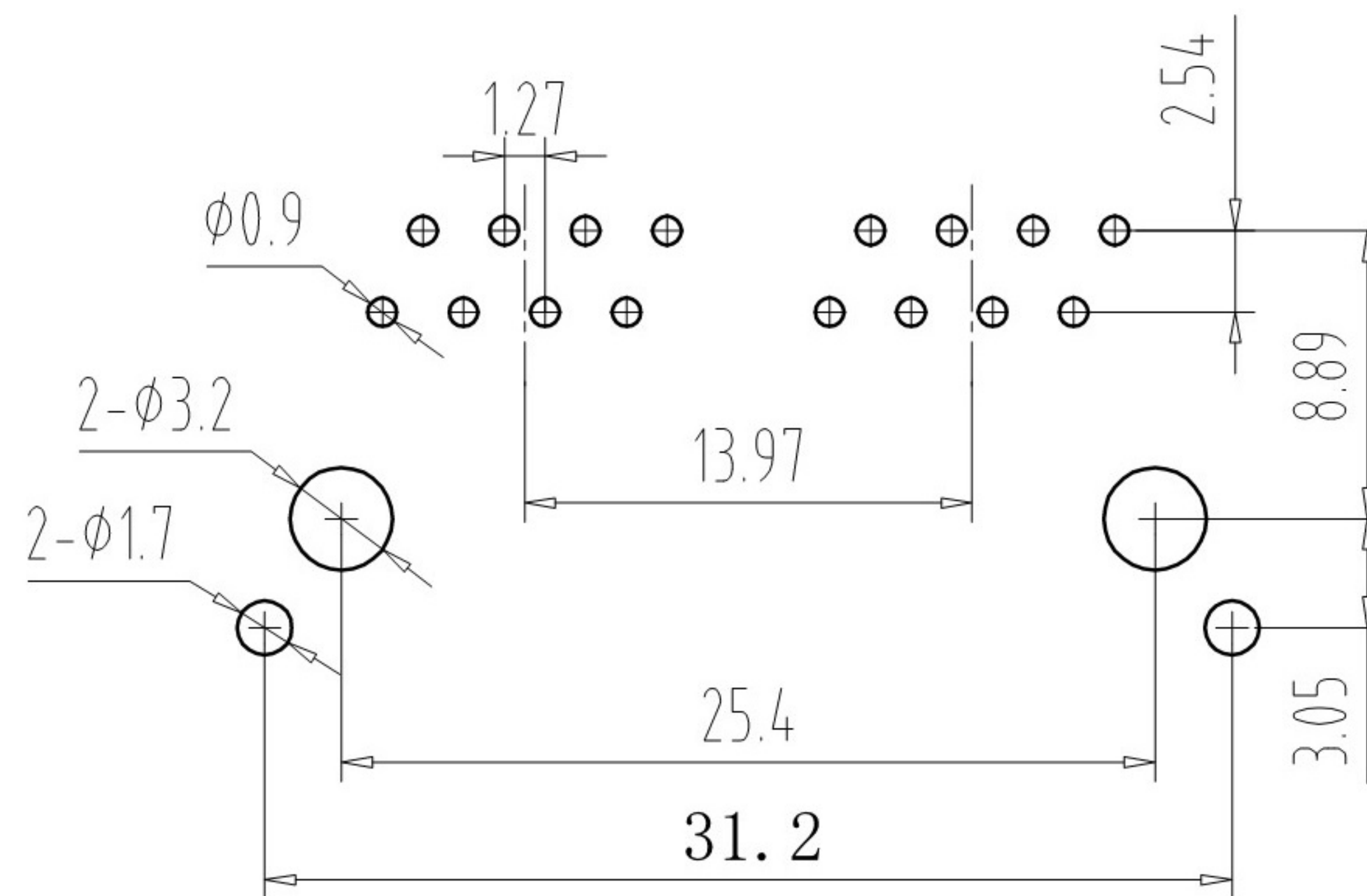
PC Board Layout Component Side Shown
