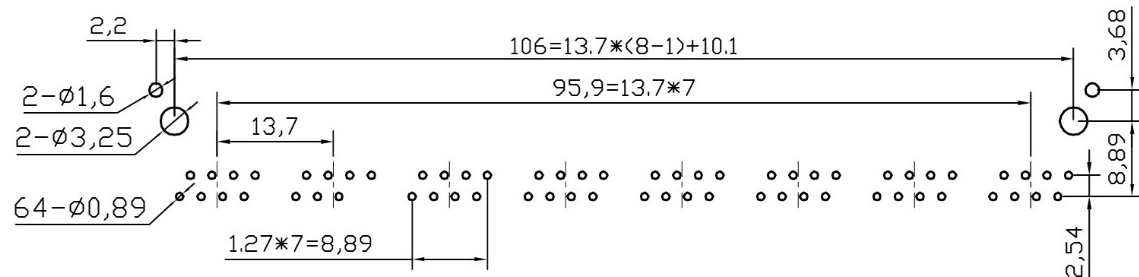
PC Board Layout Component Side Shown
