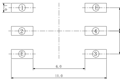
PCB WELDING DIMENSIONS
