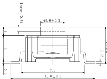
REFERENCE DRAWING
