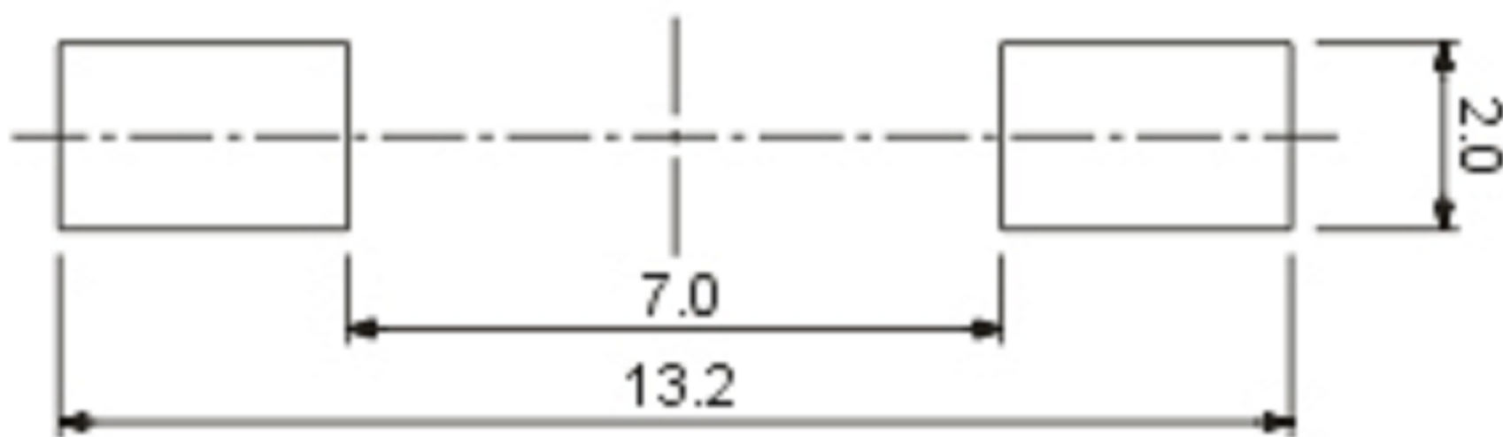
PCB LAND DIMENSION
