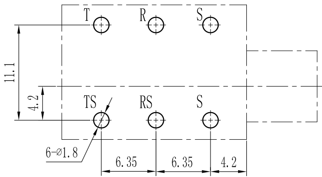
P.C.B LAYOUT (BOTTOM VIEW) Tolerance: ±0.05
