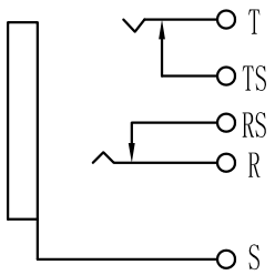
Electrical schematic
