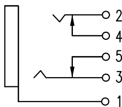
Electrical schematic
