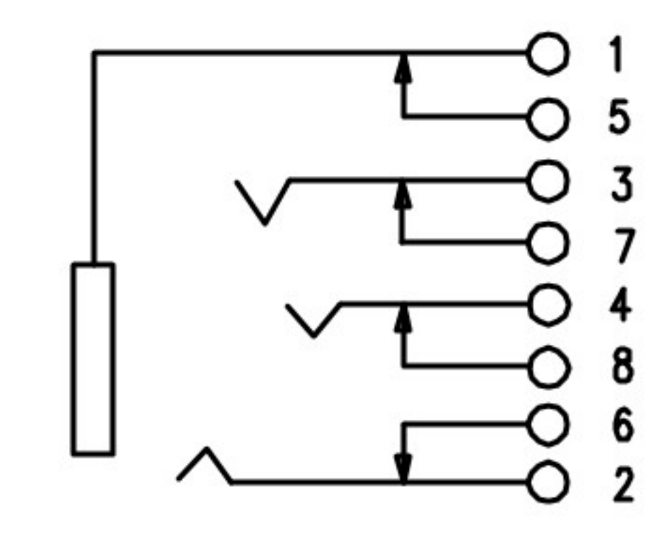
CIRCUIT DIAGRAM
