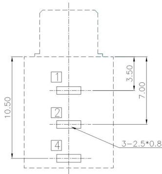
P.C.B LAYOUT(copper-sided view)
