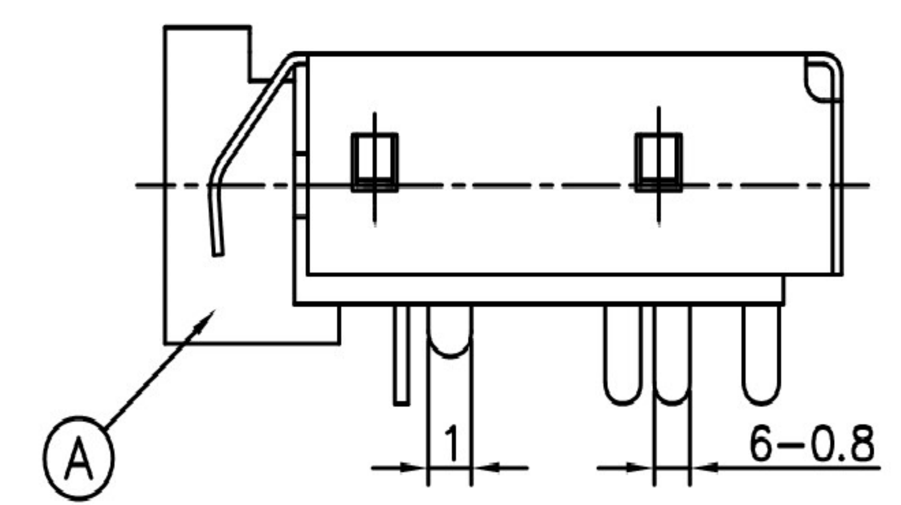
PCB MOUNTING HOLES BOTTOM VIEW (TOLERANCE: ±0.05)
