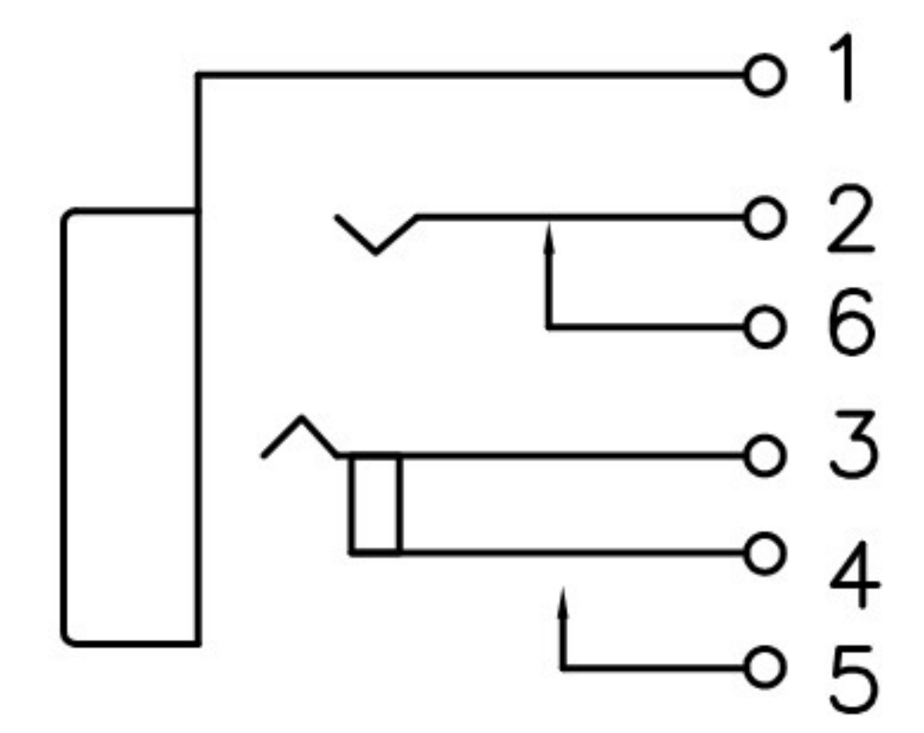
SCHEMATIC
