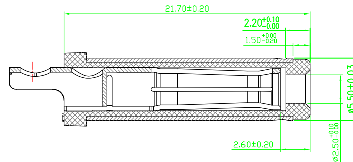
MATING PLUG DP550250-0188-60000H
