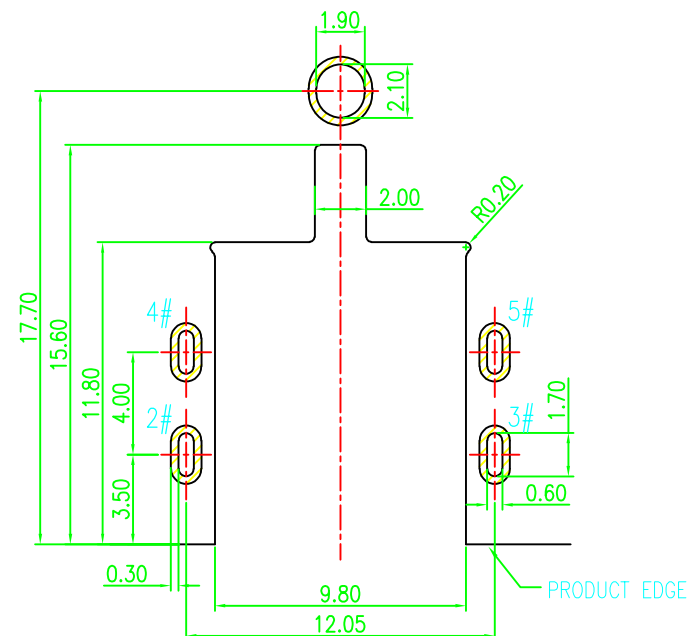
RECOMMENDED PCB LAYOUT TOP VIEW TOLERANCE: ±0.05
