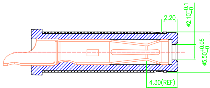
MATING PLUG DP550200-0129-60000H
