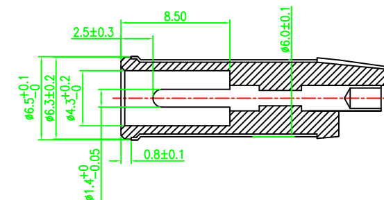
MATING PLUG
