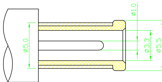
DC MATE PLUG
