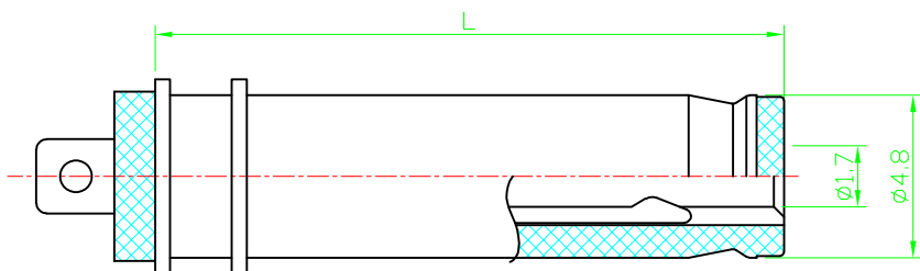
RECOMMENDED PLUG
