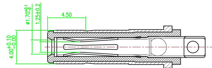
MATING PLUG DP400170-0038-60000H
