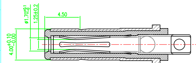
MATING PLUG DP400170-0038-60000H
