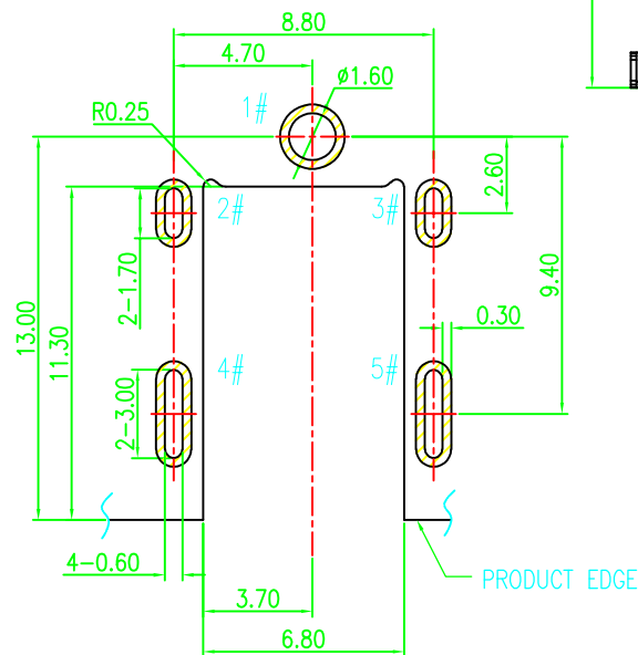
RECOMMENDED PCB LAYOUT TOP VIEW TOLERANCE: ±0.05
