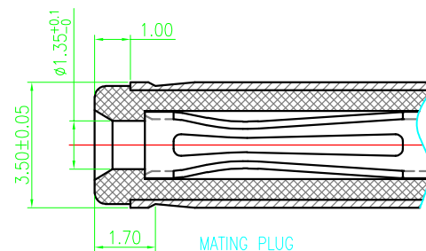
MATING PLUG
