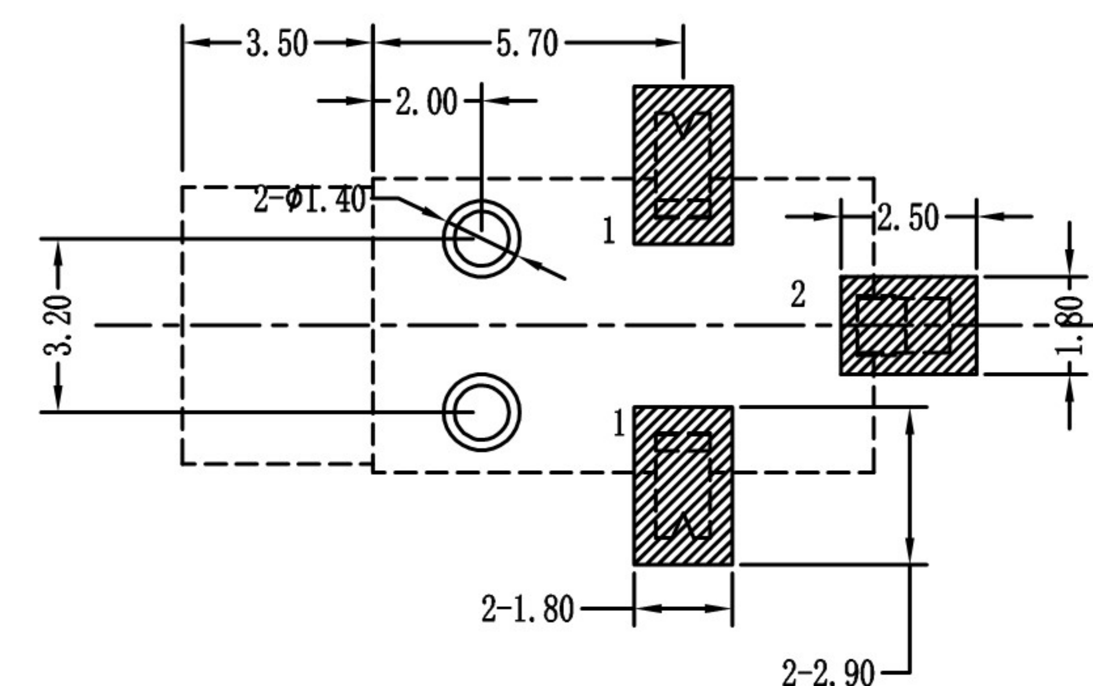
PCB LAYOUT TOP VIEW
