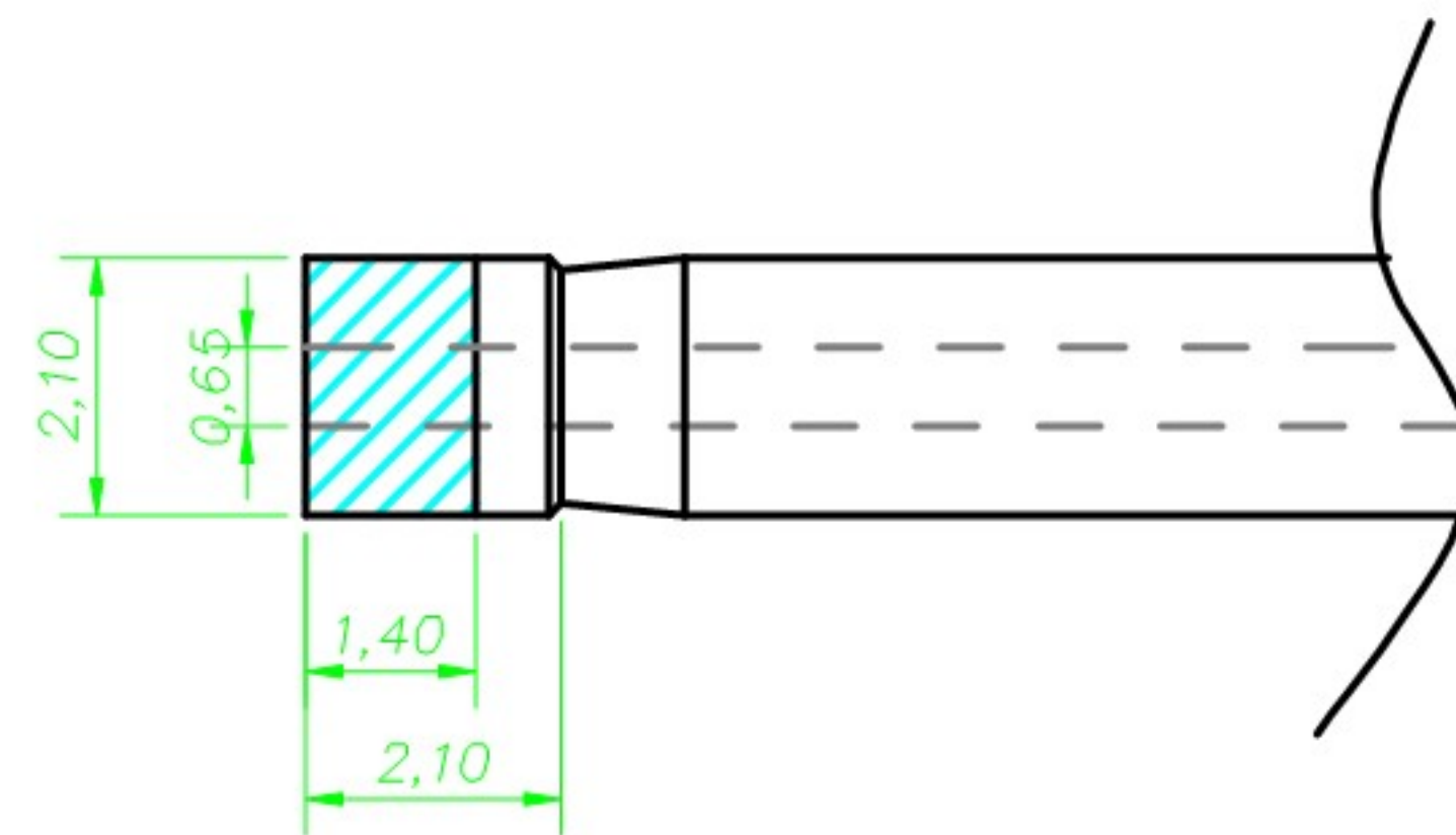
PLUG SPEC
