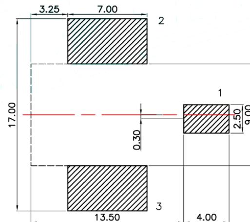
P.C.B LAYOUT(Copper-side view)
