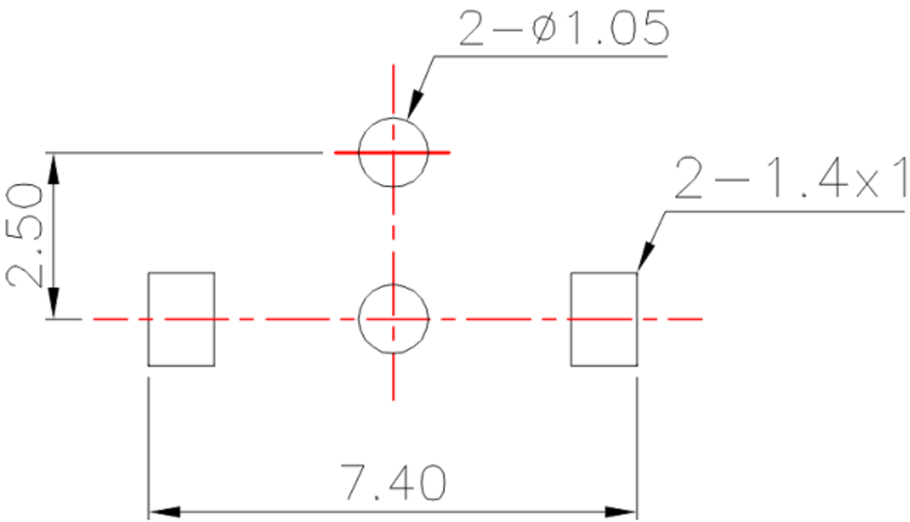
HOLE LAYOUT
