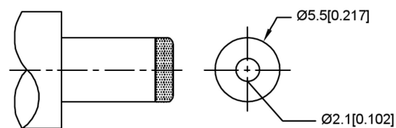
MATING PLUG Jack Insertion Depth: 9.0 mm
