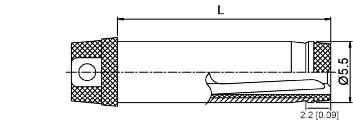
RECOMMENDED PLUG
