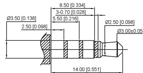
(Ø3.50mm 4 POLE PLUG DETAIL DRAWING)
