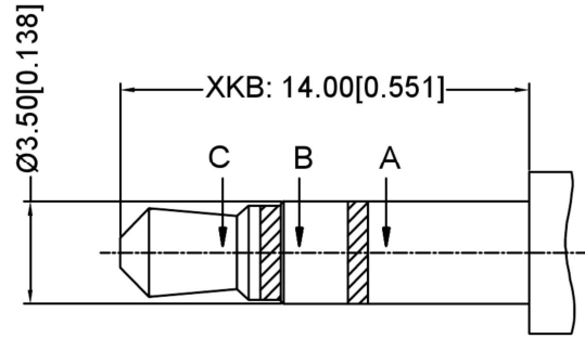
MATE PLUG
