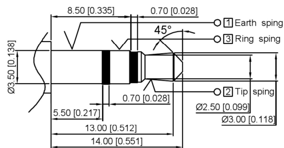
Matching Plug
