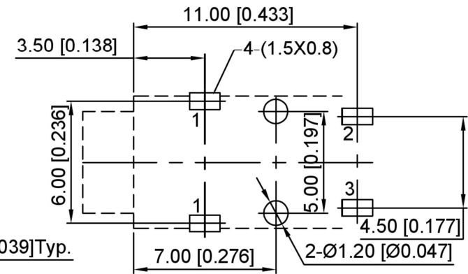
P.C.B LAYOUT MOUNTING PATTERN (TOP VIEW)
