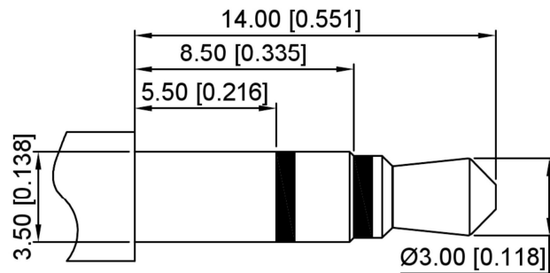
Ø3.50mm 3 POLE PLUG
