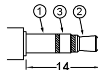
Ø3.5 MATING PLUG
