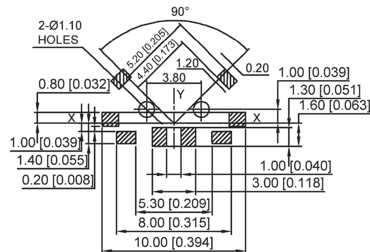
P.C.B Mounting Pattern Dimension
